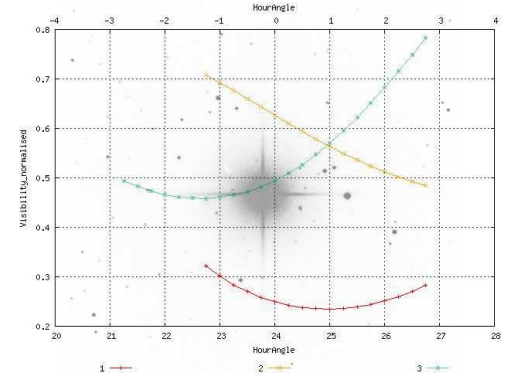
Fig. 1: This image shows the visibility values that can be measured for the planet host star \epsilon Tau using the baseline A0-K0-G1 at hour angles between -3h and +3h
