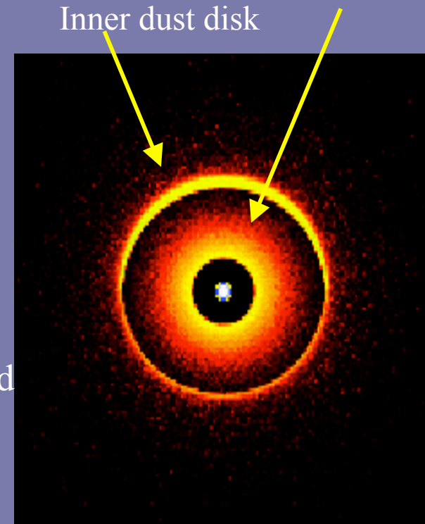
K band model image, 1 AU across
