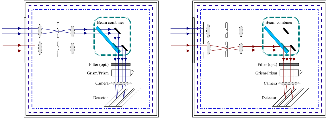
Fig. 4. MIDI optical configuration for the photometric calibration of the visibility that is performed before or after the fringe record in High-Sens mode. In order to keep the optical configuration identical to the one for the fringe record, the beam combiner is kept and a shutter allows us to select one of the telescope. The two cases are shown in order to ease the understanding of the way MIDI creates the fringes, and the origin of the 90 degree flip between the two interferometric outputs (from Ratzka PhD Thesis).
