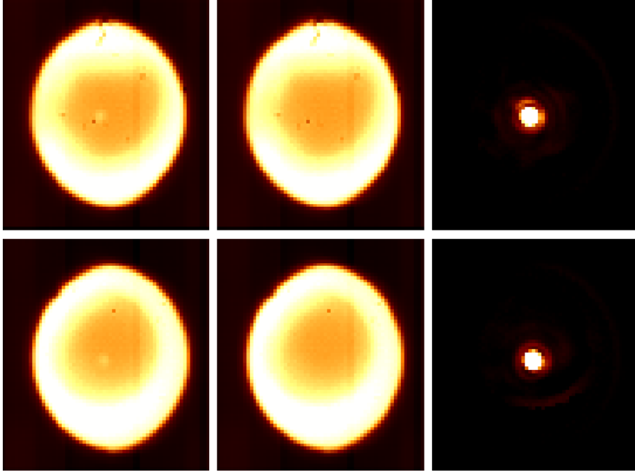
Fig. 3. Example of chopping data for a bright source ( F=140\text{Jy} , m_N=-1.4 ). The mean of the on-source frames (left), the mean of the off-source frames (centre), and their difference (right) is shown for UT3 (upper row) and UT4 (lower row). Three Airy rings are visible in the upper right image. The bright external regions originate from the tunnels background emission while the darker area delimits the sky background, at colder temperature and less emissive. This dark area is indeed the larger Field-Of-View of the VLTI/MIDI instrument possible from sky acquisition. Note the different shapes and sizes of this FOV for each telescope due to alignment and technical problems (i.e. current absence of variable curvator mirrors). These shapes and sizes depend on the sky position of the source and evolve with time.
