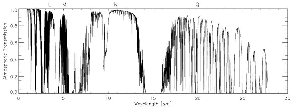
Fig. 1. Atmospheric transmission in the mid-infrared (from Ratzka PhD thesis). Note the broadness and cleanness of the N band compared to other bands. The spectral limits in which MIDI provides good quality data are usually between 7.8 and 13.5 micron. Note also the strong decrease of the atmospheric transmission in the ozone band at 9.7\mu\text{m} .
