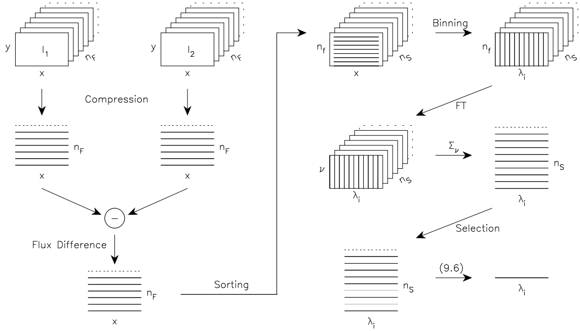
Fig. 5. MIA software algorithm (from Ratzka PhD Thesis) . In a first step two Gaussian masks are created that suppress the areas that lie outside of the central region and are only illuminated by the background. The next steps after multiplying the n_F interferometric frames of I_1 and of I_2 with the masks are schematically presented in this figure. Compression: The frames are compressed in the spatial( y )-direction, i.e. the n_F two-dimensional images in both stacks are transformed into n_F one-dimensional arrays. Flux Difference: The one-dimensional arrays originating in beam I_2 are subtracted from those originating in beam I_1 . Sorting: The n_F (for instance 8000) one-dimensional arrays are arranged into the n_S (= 200) scans in which they have been taken, i.e. n_f = n_F/n_S (= 40) arrays belonging to one scan are handled as a unit. Binning: The x -direction, representing the wavelength, is binned by default between 8 \mu\text{m} and the 13 \mu\text{m} into stripes \lambda_i with a width of 3-4 pix. Fourier Transform: The 1-D scans are Fourier transformed and the flux of the fringe peak, corrected from the noise, is extracted. Selection: The value of the Fourier amplitude of the white-light fringe is used as criterion to decide whether a scan can be used for the determination of the correlated flux.
