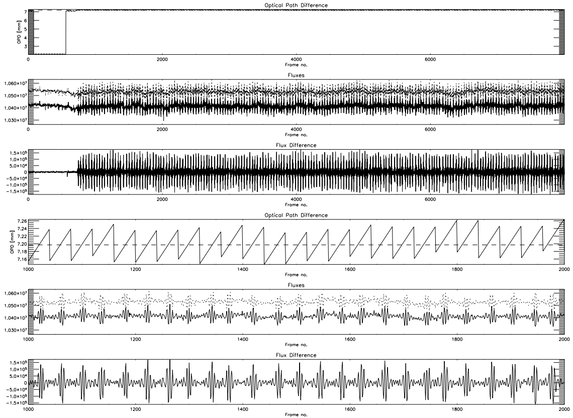
Fig. 6. Part of the MIA GUI representing from top to bottom: the OPD Panel in mm (top, abscisse axis in frame number n_F ), the level of the flux extracted for each telescope in counts, the difference of these flux illustrating the efficient removal of the background and the fringe signal in anti-phase emerging strongly, a zoomed view of the OPD Panel showing the scans of the piezo super-imposed to the OPD residuals of the tracking, the fluxes from each telescopes with the fringes in anti-phase and their difference. Figure from MIA web site and Ratzka PhD thesis.
