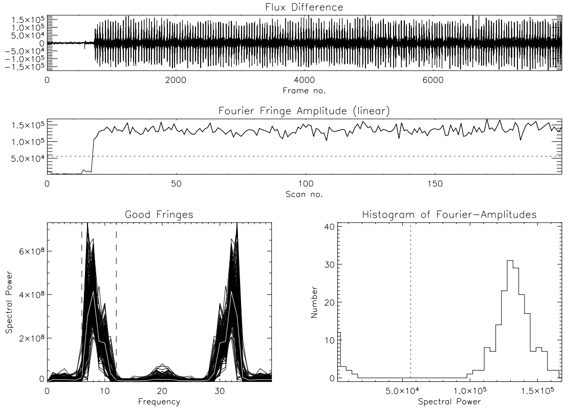
Fig. 7. Part of the MIA GUI representing the flux difference between the I1 and I2 beams in counts (top, abscisse axis in frame number n_F ), the level of the correlated flux estimated for the full N band from the Fourier transform of each scan (middle, abscisse axis in scan number n_S ), the Fourier peaks Panel (bottom left) and the Histogram of the Fourier-Amplitudes (bottom right). Figure extracted from the MIA web site.
