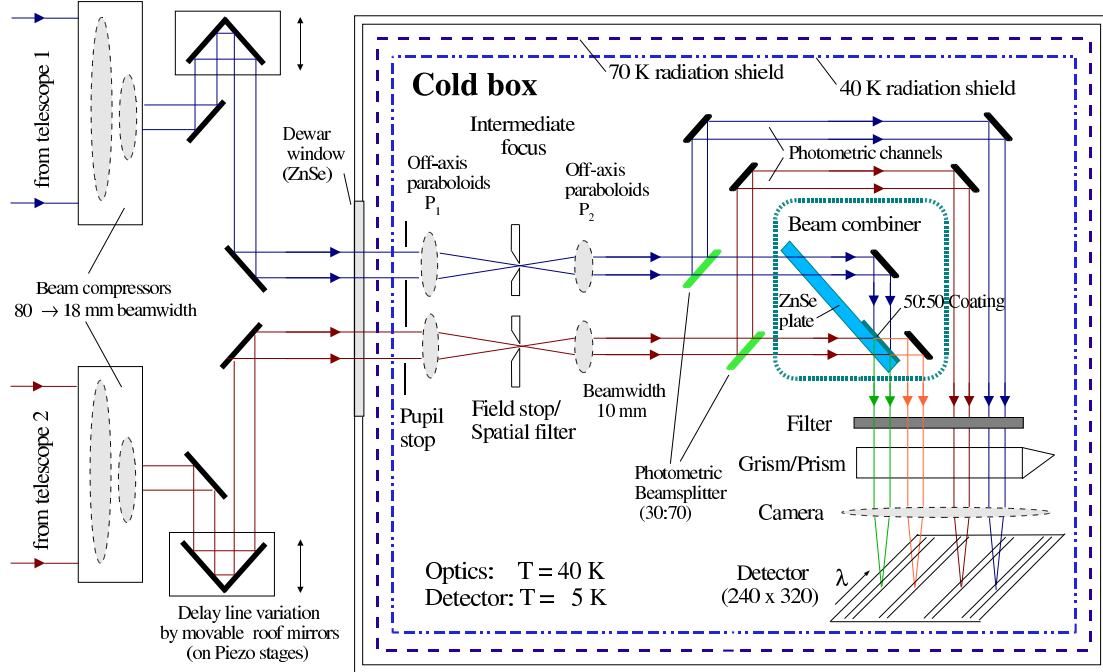
Fig. 2. Schematic optical layout of MIDI (image courtesy of U. Graser, MPIA).
